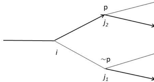
Figure 2 a Molinistic model in which the time branches at moment i and j , and where it is stipulated, with an arrow, what will be the case at j , namely p .
