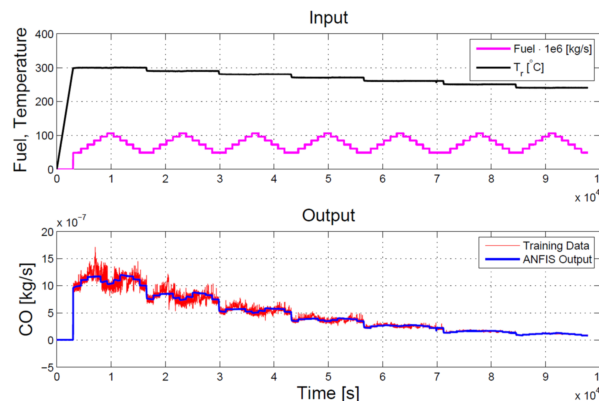
Figure 3: Output of ANFIS model for carbon monoxide content in the reformat gas. Inputs are reformer temperature, T_r , and the fuel flow.
