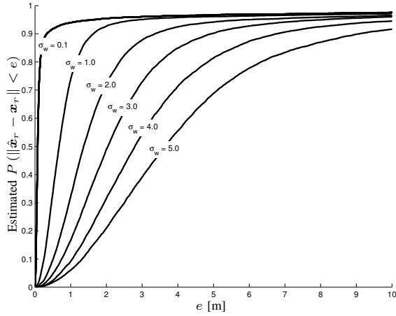
Figure 7. Estimated cumulative localization error probability at iteration 100 with \sigma_w as a parameter based on 100 independent simulation runs.
