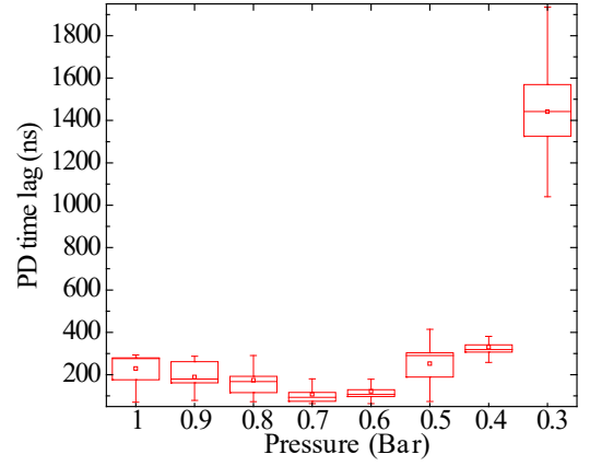
Fig. 17. PD time lag under different pressures
