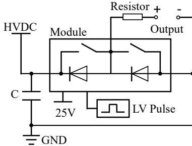
Fig. 3. Pulse voltage generator based on a half bridge power electronic power module
