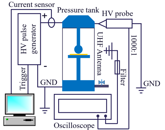
Fig. 10. Test system
