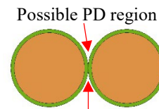
Fig. 2. Possible PD region in the winding of the transformer: (a) With additional inter layer/winding insulation. (b) Without additional inter layer
