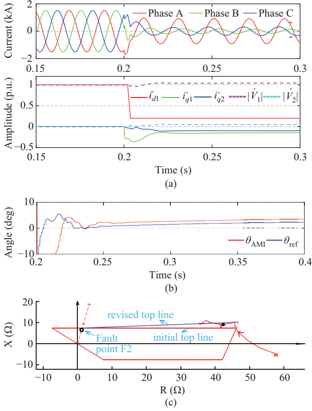
Fig. 11. Fault AG at F2 ( R_f = 40 \Omega ). (a) Fault currents and control signals. (b) Dynamic angles \theta_{\text{AMI}} and \theta_{\text{ref}} . (c) Trajectory of Z_{\text{app}}^{\text{AG}} .
