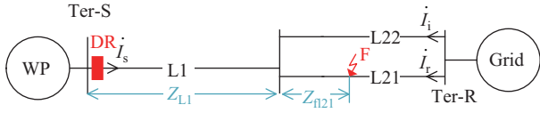
Fig. 10. Single-line fault diagram of WP outgoing system for the fault on L21.
