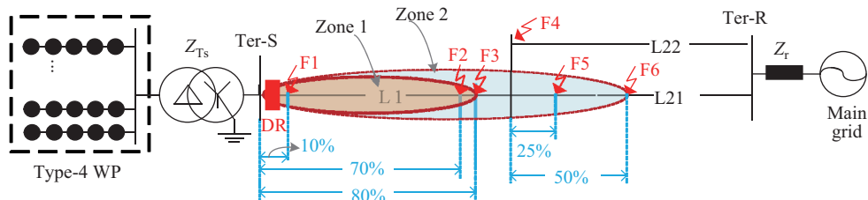
Fig. 6. Type-4 WP outgoing test system.
