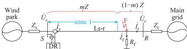
Fig. 1. Single-line diagram of the fault network connecting type-4 WP.
