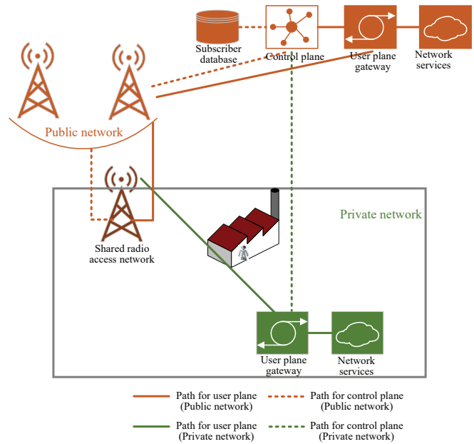
Fig. 3. Deployment with shared RAN and control plane. (Adapted from [14])
