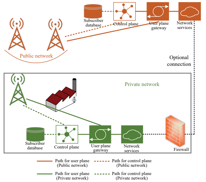
Fig. 1. Deployment as isolated network. (Adapted from [14])
