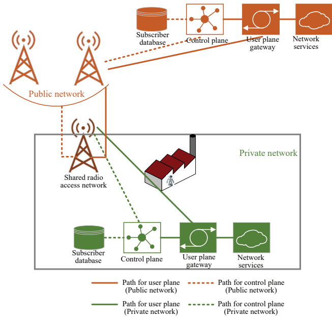
Fig. 2. Deployment with shared RAN. (Adapted from [14])
