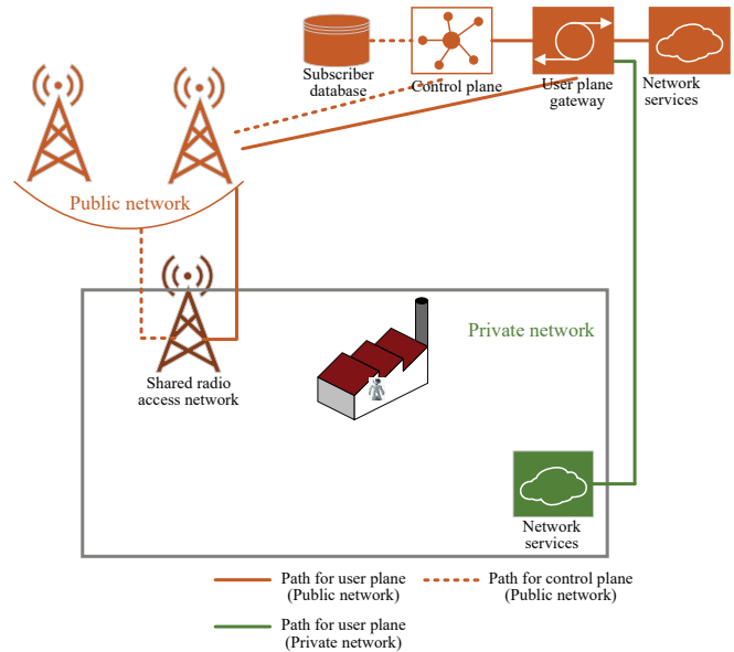
Fig. 4. Deployment in a public network. (Adapted from [14])
