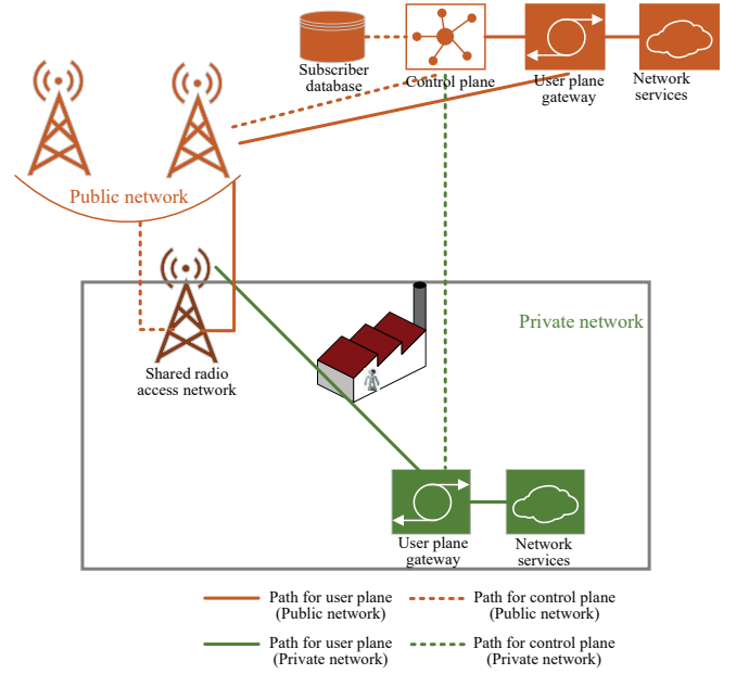
Fig. 3. Deployment with shared RAN and control plane. (Adapted from [14])
