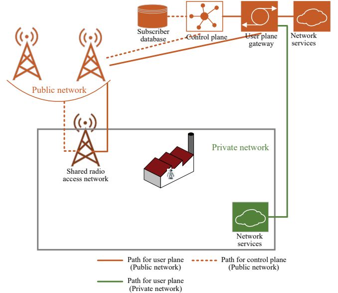
Fig. 4. Deployment in a public network. (Adapted from [14])
