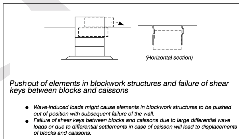
Figure VI-2-62. Displacement of individual blocks
