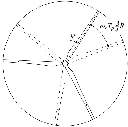
Fig. 5. LIDAR measurement positions (crosses) in the rotor plane. Measurements are taken \omega_r T_p radians ahead of the blades and at 75 % blade span.
