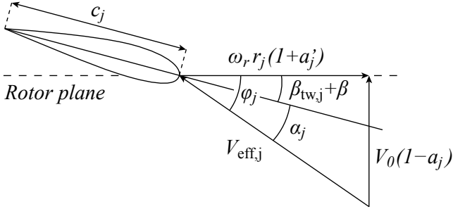
Fig. 2. Wind components and angular quantities for blade element j .
