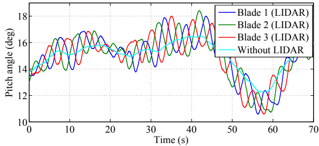
Fig. 8. Comparison of pitch activity from 0 s to 70 s.
