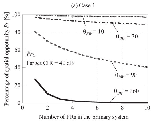
Fig. 13 Percentage for spatial opportunity versus the number of primary receivers (PRs).
