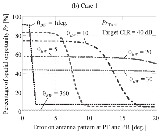
Fig. 12 Percentage for spatial opportunity when the error on the beam pattern exists.
