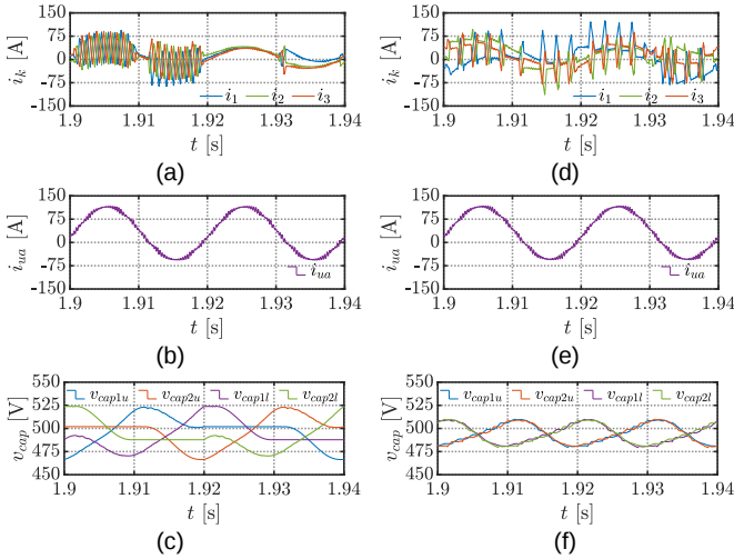
Fig. 5. Interleaved leg currents in one submodule of ISM-MMC (a,d), the corresponding arm current (b,e) and capacitor voltages in phase ‘a’ of ISM-MMC (c,f) at sorting frequency 50 Hz (a,b,c) and at 1 kHz (d,e,f).
