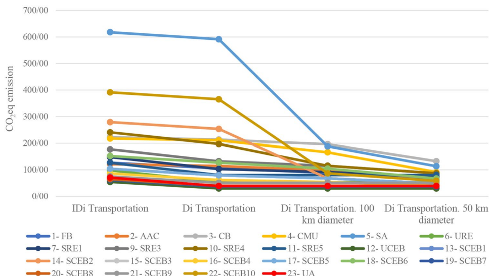
Fig. 9 CO 2 eq emissions from the transportation stage sensitivity analysis (A4)
