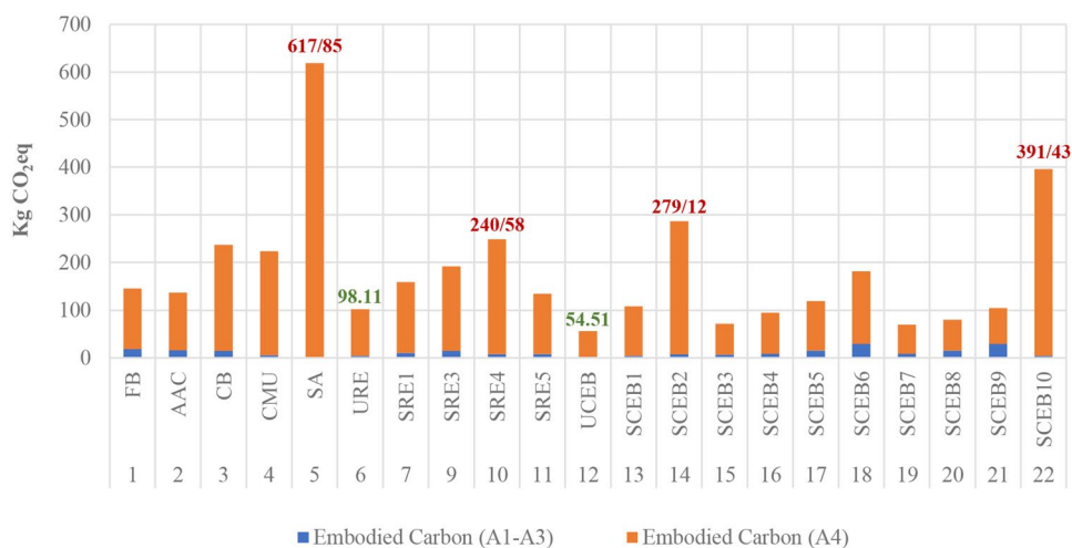
Fig. 5 CO 2 eq emissions emitted per each life cycle stage for each wall assembly (A1–A3 and A4)
