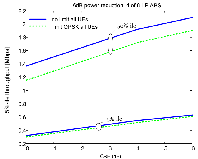
Figure 7. 5%-ile and 50%-ile experience user throughput with modulation constraint
