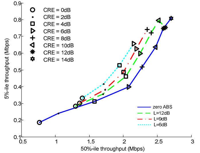
Figure 3. 5%-ile vs 50%-ile experience user throughput with ABS and LP-ABS and different CRE offsets
