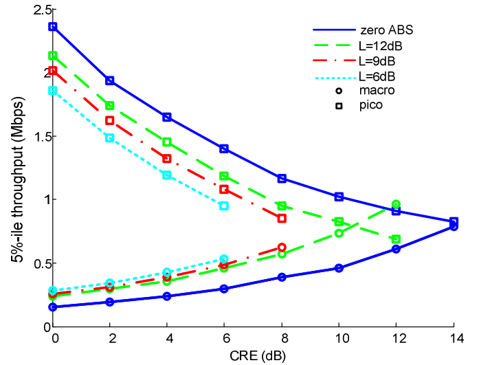
Figure 4. Macro and pico 5%-ile performance for ABS and LP-ABS
