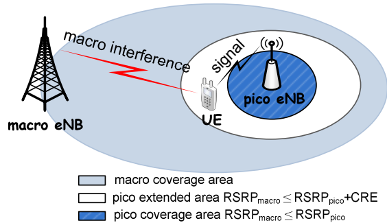
Figure 1. Baseline macro-pico heterogeneous network.
