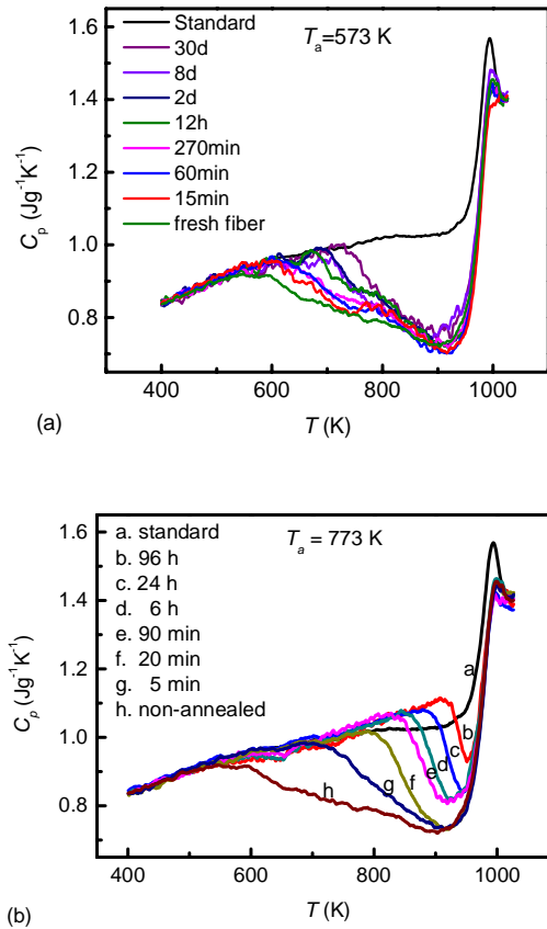
Figure 5-2. Isobaric heat capacity curves for the hyperquenched (HQ) sample, the sample cooled at 20 K/min, and the samples hyperquenched and subsequently annealed (AHQ) for various durations at the annealing temperatures ( T_a ): (a) 573 K; (b) 773 K.
