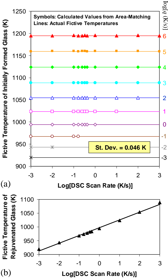
Figure 4-5. (a) Results of T_{fi} calculations using the simulated DSC with initial cooling rates between 10^{-3} and 10^6 K/s and scan rates between 10^{-3} and 10^3 K/s. The derived values of T_{fi} using area-matching (symbols)
