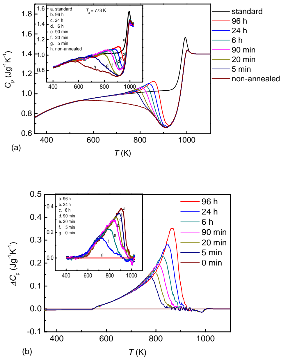
Figure 6-7. (a) Modeled heat capacity curves of basalt fibers annealed at 773K for different duration with the experimental data inserted. (b) Heat
