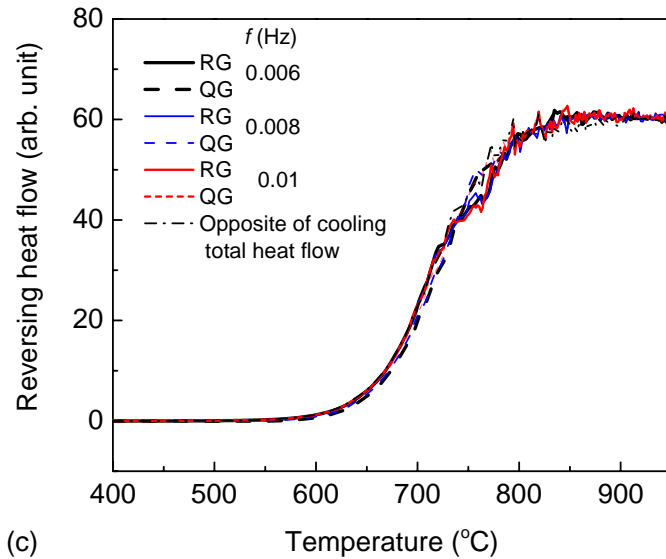
Figure 3-3. The reversing heat flow with frequency ( f ) correction: (a) rejuvenated glass (RG) showing a master curve for f = 0.002, 0.003, 0.004, 0.006, 0.008, 0.01 Hz; (b) quenched glass (QG) showing a master curve for f = 0.006, 0.008, 0.01 Hz; (c) rejuvenated glass (RG) and quenched glass (QG) for f = 0.006, 0.008, 0.01 Hz and the opposite of the total heat flow in cooling (The heat flow in cooling is exothermic, other than endothermic in heating. In order to see how
