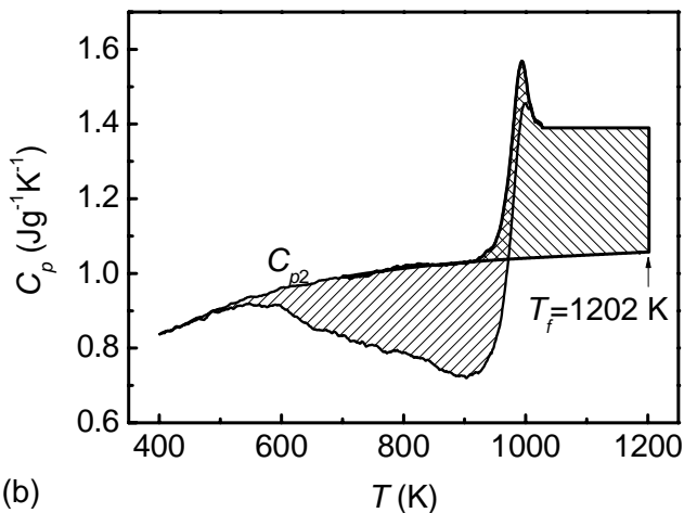
Figure 5-1. (a) Determination of T_g for the standard sample that was reheated to above the glass transition and subsequently cooled at 20 K/min. (b) Determining T_f of the hyperquenched (HQ) (as-produced) sample, where C_{p2} is the isobaric heat capacity for the sample cooled at 20 K/min. The uncertainty of T_f determined by DSC measurement is about 1%.
