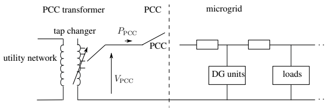
Fig. 9. Smart transformer in microgrid
