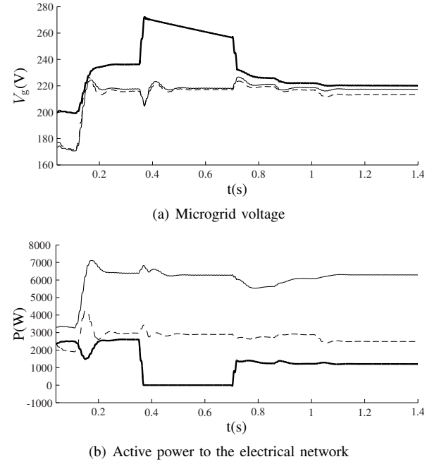
Fig. 19. Dynamic profile: without smart transformer (— = VSI 1; ---- = VSI 2; —·— = VSI 3)
