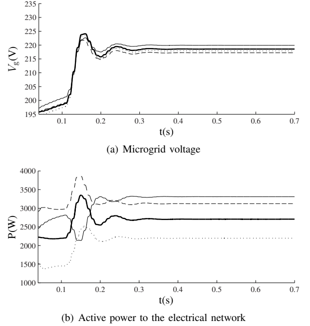
Fig. 16. Smart transformer in microgrid: without smart transformer (— = VSI 1; ---- = VSI 2; — = VSI 3, ... = VSI 4)
