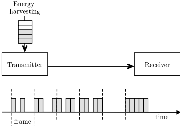
Fig. 2. Communication system with energy harvesting and ON/OFF signaling. The frame size if F = 5 .
