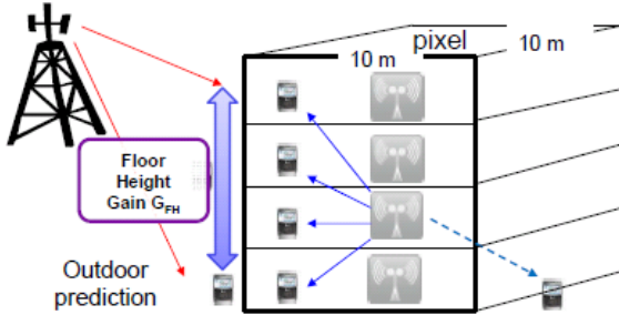
Figure 2. Outdoor-Indoor Floor Height Gain and 3D user distribution
