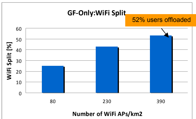
Figure 9. Wi-Fi deployment: % offloaded users vs. AP Density
