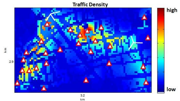
Figure 3. Overview of outdoor pico(A) deployment over traffic spatial distribution with 70/30 indoor to outdoor traffic split.
