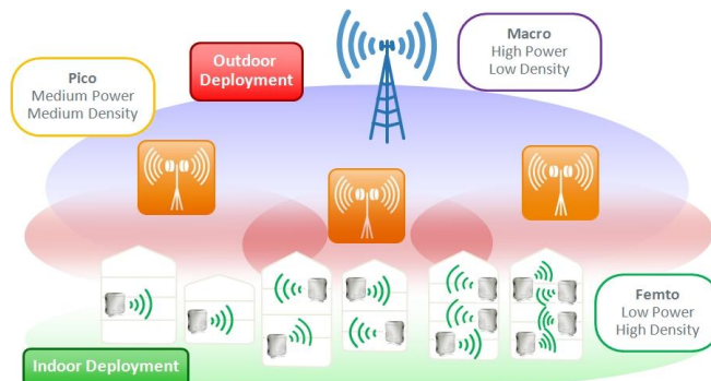
Figure 1. Overview of a multi-layer deployment scenario including outdoor macro and pico cells together with femto indoor deployment.
