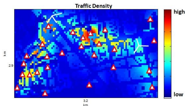
Figure 3. Overview of outdoor pico(A) deployment over traffic spatial distribution with 70/30 indoor to outdoor traffic split.
