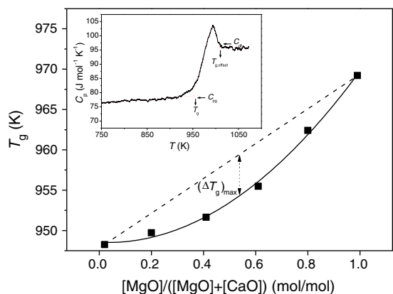
Fig. 10. The glass transition temperature from differential scanning calorimetry as a function of the molar ratio of [\text{MgO}] / ([\text{MgO}] + [\text{CaO}]) . The solid line represents the apparent relation between T_g and the molar ratio of [\text{MgO}] / ([\text{MgO}] + [\text{CaO}]) , whereas the dashed line is a linear relation; both are guides for the eye. (\Delta T_g)_{\text{max}} is marked on the figure where the largest discrepancy exists between linear relation and apparent relation, i.e., the largest mixed alkaline earth effect. Inset: Method for determining T_g and characteristic heat capacities from the heat capacity curves measured by differential scanning calorimetry [53]. The uncertainty of this method is \pm 2\text{--}3 \text{ K} [88].
