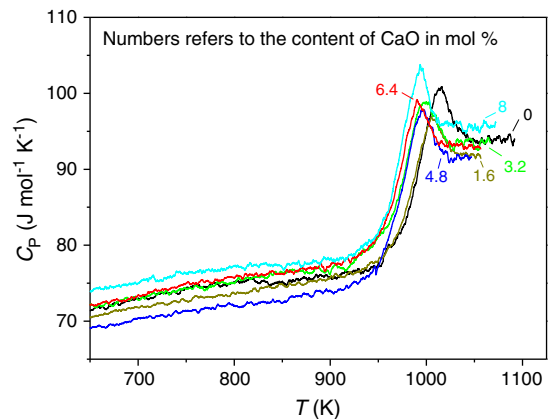
Fig. 8. Heat capacity as a function of temperature for the six samples with different CaO contents (in mol%) as indicated in the figure. The composition of each sample is given in Table 1. The heat capacities are determined by differential scanning calorimetry at a heating rate of 10 K/min subsequent to a cooling of 10 K/min.
