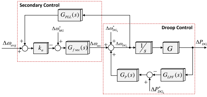
Fig. 7. Small signal model of distributed frequency control for a DG unit in a low R/X islanded MGs.
