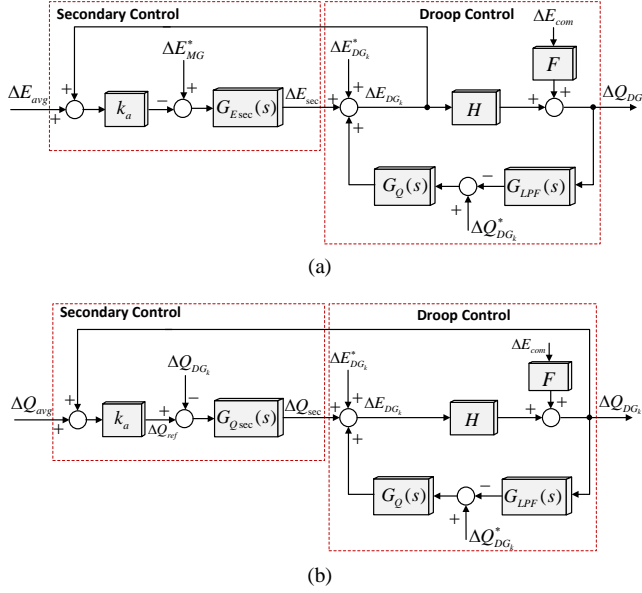
Fig. 9. Small signal model of distributed control for a DG unit in a low R/X islanded MicroGrids a) voltage control b) reactive power sharing.
