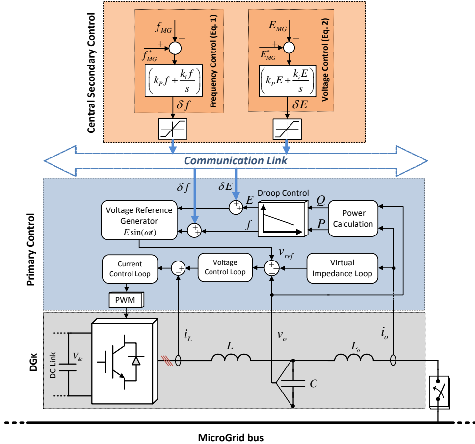
Fig. 3. Scheme of the central secondary control for a DG unit in a MG.
