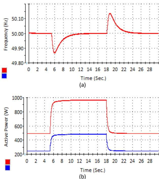
Fig. 14. Performance of the DSC for an islanded MG consists of two DGs with different power rates. a) Frequency b) Active power. DG1 (blue), DG2 (red).
