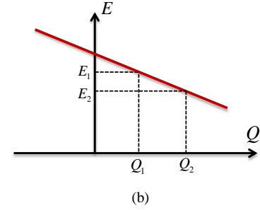
Fig. 8. Q-E droop control problem in reactive power sharing.
