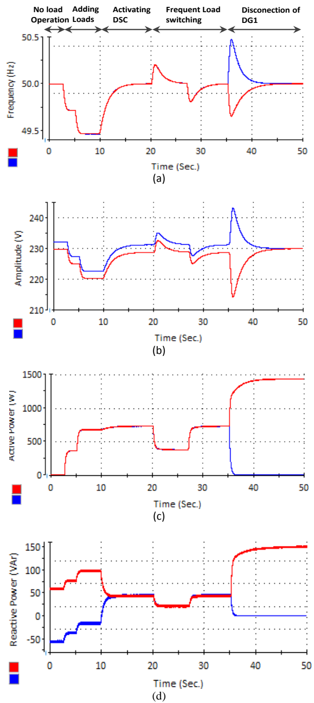
Fig. 13. Performance of DSC in a) frequency restoration b) voltage amplitude restoration c) active power sharing d) reactive power sharing. DG1 (blue), DG2 (red).
