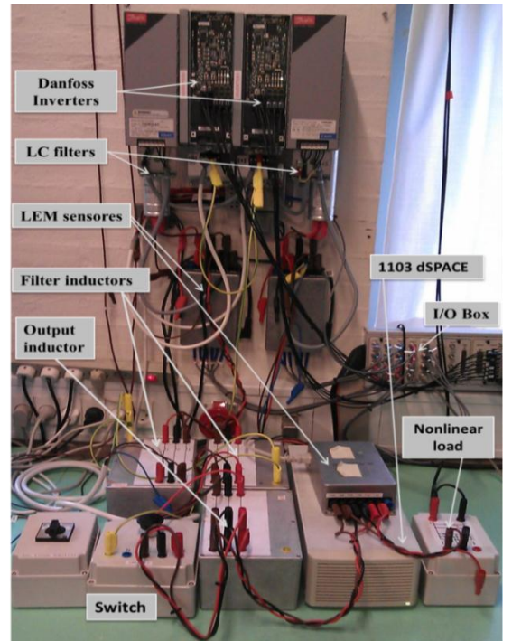
Fig. 11. Experimental setup.
