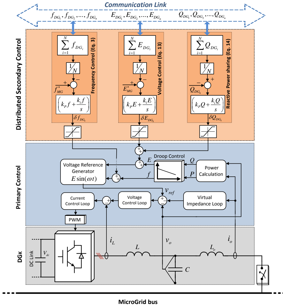
Fig. 5. Scheme of the proposed distributed secondary control for a DG unit in a MG.
