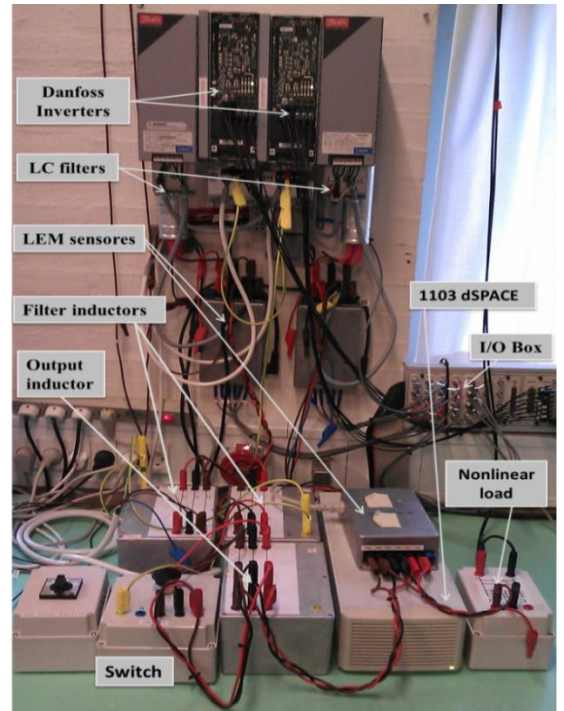
Fig. 11. Experimental setup.
