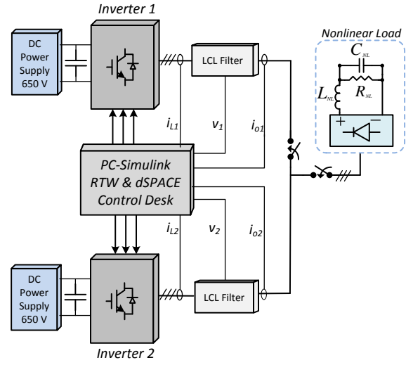
Fig. 10. Schematic of Experimental setup.
