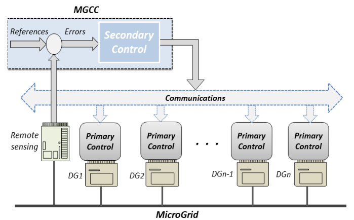
Fig. 2. Centralized secondary control.
