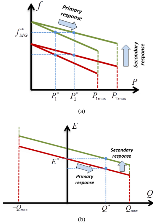
Fig. 6. Secondary control response vs primary control response. (a) frequency restoration (b) Voltage amplitude restoration.
