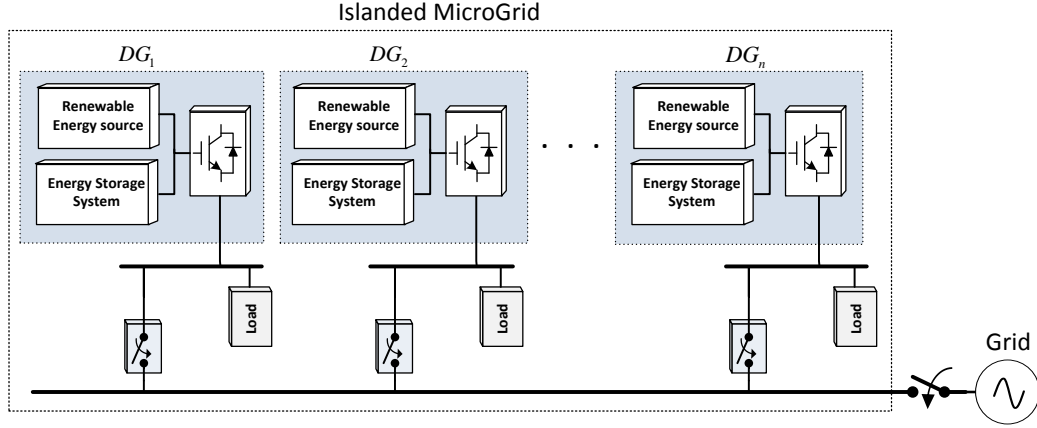
Fig. 1. General structure of MG.
