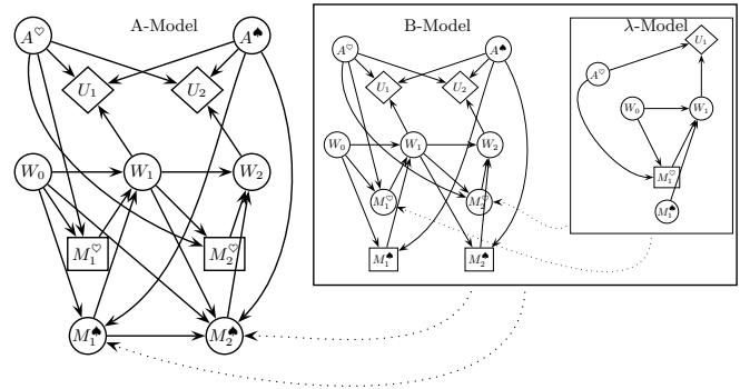
Figure 1: An ID framework for opponent modeling which contains a set of nested models. This one has nesting level 3 and time horizon 2
