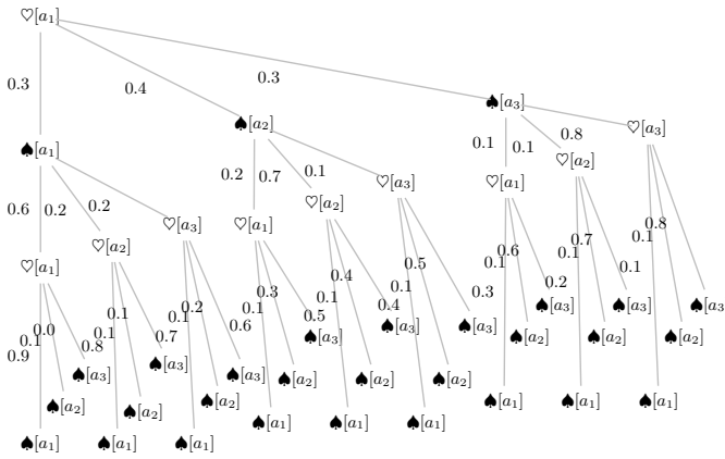
Figure 2: The tree representing the level 3 initial type for ♡. ♡ knows her own assignment a_1 . From the root there is a branch to a sub tree for each possible ♠ assignment. The edges are labeled with the probability assigned to each subtree.
