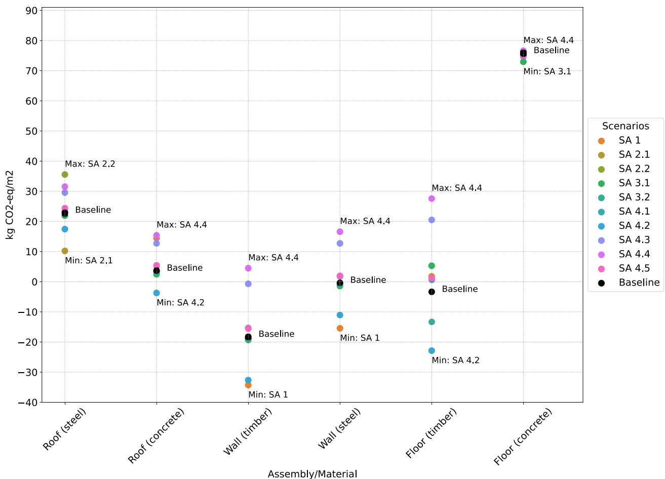
Fig. 7 Sensitivity analysis results for each assembly (sLCA method), highest and lowest sensitivity analysis results individually labelled for each assembly (including module D)
