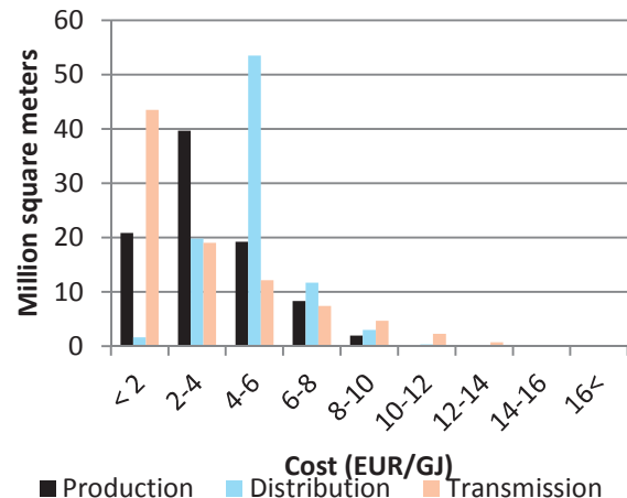
Figure 7: Potential outside (energy quality method and no heat savings)
