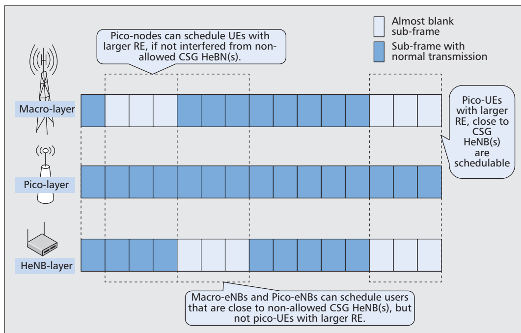
Figure 2. Basic principle of TDM eICIC for LTE-Advanced.
