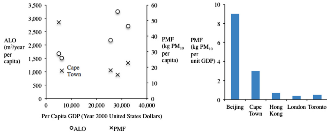
Figure 5. Per capita ALO as \text{m}^2 \text{yr}^{-1} and PMF as \text{kg particulates} < 10 \mu\text{m yr}^{-1} are shown on the left. Local air pollution issues in Beijing and Cape Town are disproportionately high relative to the amount of economic activity, particularly when the IP per unit of economic activity is taken into account as shown on the right. Wealthier cities show a tendency to minimize air pollution while the exported environmental pressure of ALO increases with the wealth of the residents.
