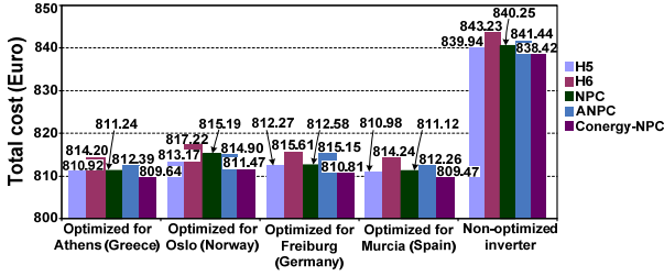
Fig. 5. The total cost of the optimized and non-optimized H5, H6, NPC, ANPC and Conergy-NPC PV inverters for various installation sites in Europe.
