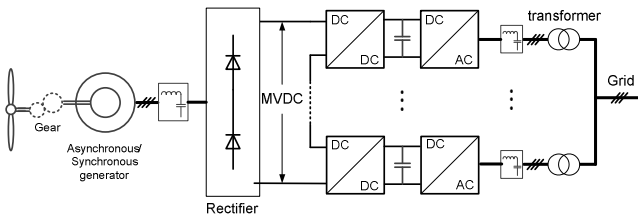
(c) Multi-cell converters with generator side series and grid side paralleled (Series-Parallel).
