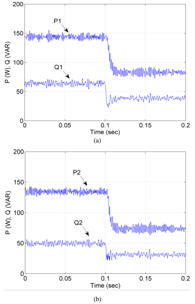
Fig. 12. Experimental dynamic response when the load demand decreased, (a) DG1 output powers, (b) DG2 output powers.
