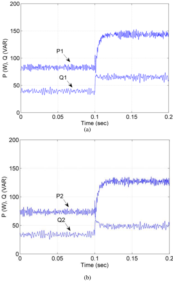
Fig. 11. Experimental dynamic response when the load demand increased, (a) DG1 output powers, (b) DG2 output powers.
