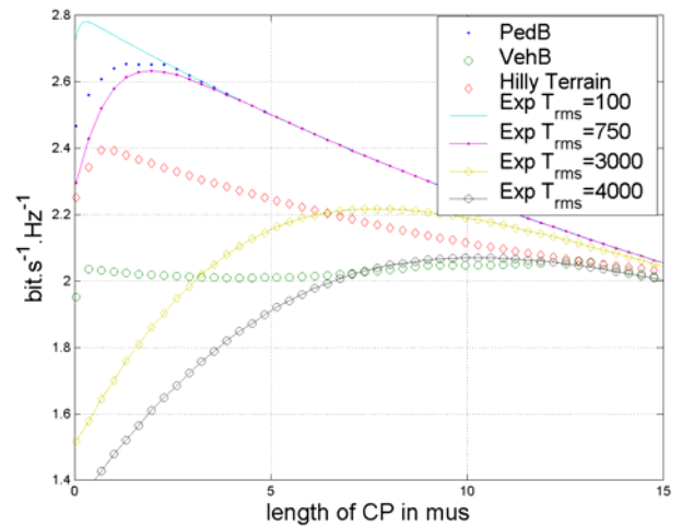
Figure 5: Capacity vs. CP length for an exp. PDP with increasing T_{rms} , SNR=15dB, T_s = 40 \mu s.
