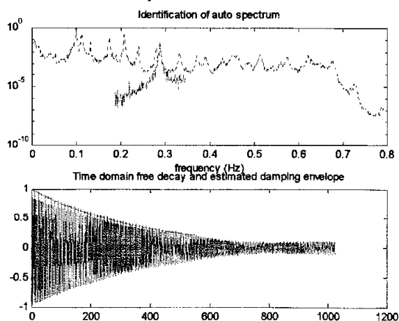
Figure 10. Partially identification of auto spectral density associated with a closely spaced mode.
