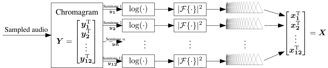
Figure 1. Block diagram of the feature extraction.
