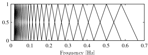
Figure 4. Bandwidths of the 25 logarithmically spaced filters.
