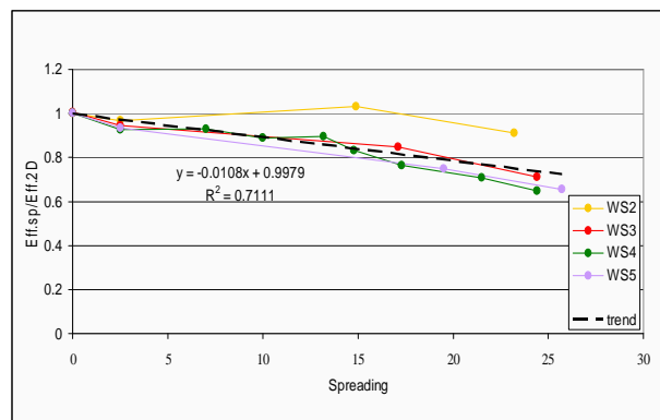
Figure 11. Influence of spreading on the hydraulic efficiency.
