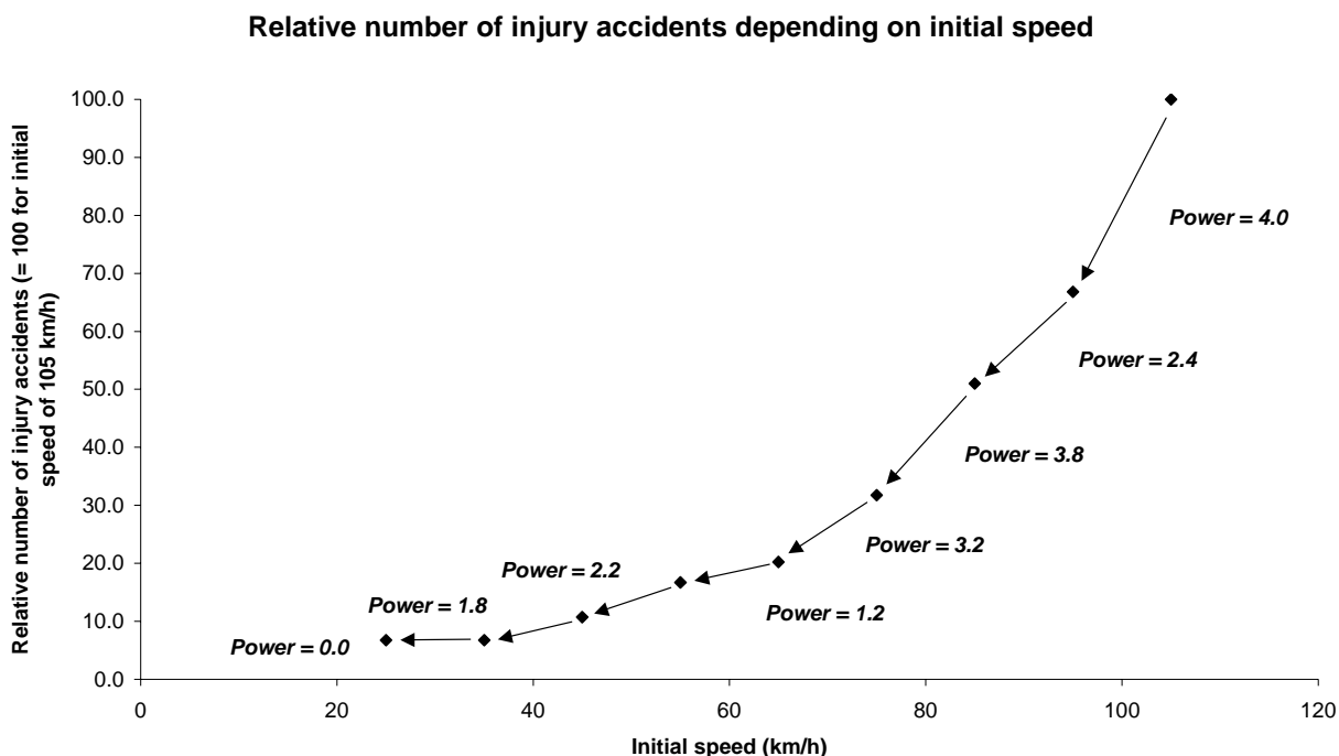
Figure 21: Relative number of injury accidents, depending on initial speed
