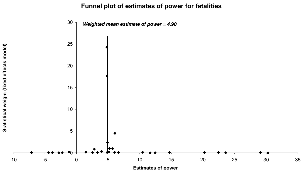
Figure 15: Funnel plot of estimates of power for fatalities
