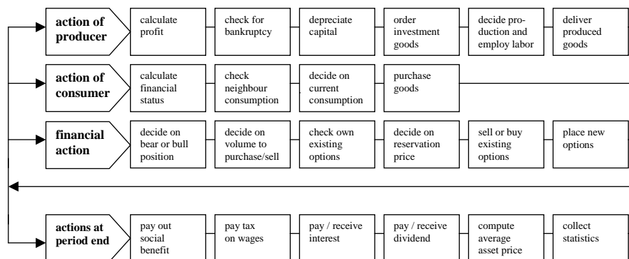
Figure 1: Decision procedures.
