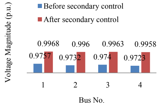
Fig. 4 Voltage profile comparison before and after secondary control
