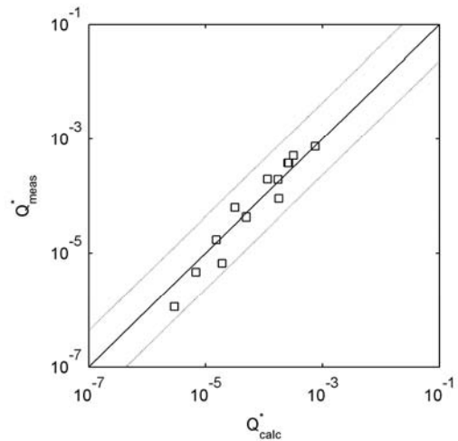
Figure 14: Evaluation of present overtopping formula against data by Porarinsson (2004).
