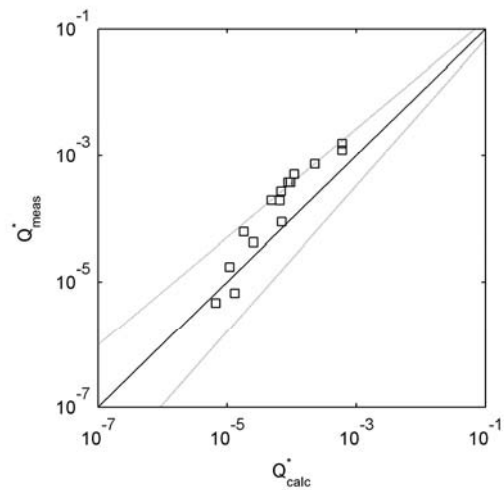
Figure 20: Evaluation of CLASH NN-Model against data by Porarinsson (2004).
