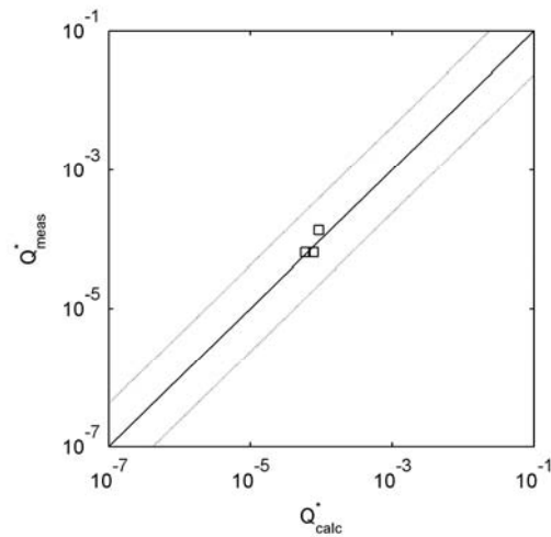
Figure 4: Evaluation of present overtopping formula against data by Bolatti Guzzo and Marconi (1991).
