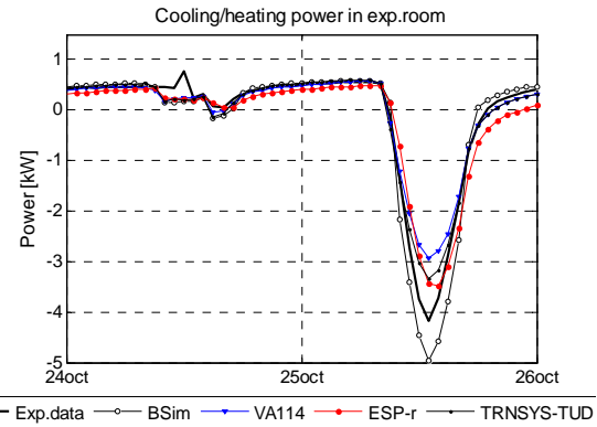
Figure 7. Cooling/heating power in the experiment room. DSF100_e.
