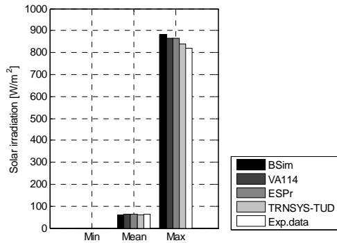
Figure 5. Total solar radiation on the external DSF surface. DSF100_e.
