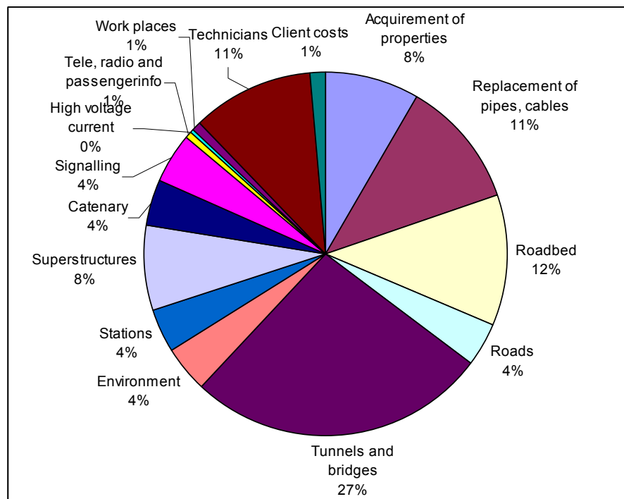
Figure 17. Relative cost distribution on main accounts (Based on data form the Danish Transport Authorities).
