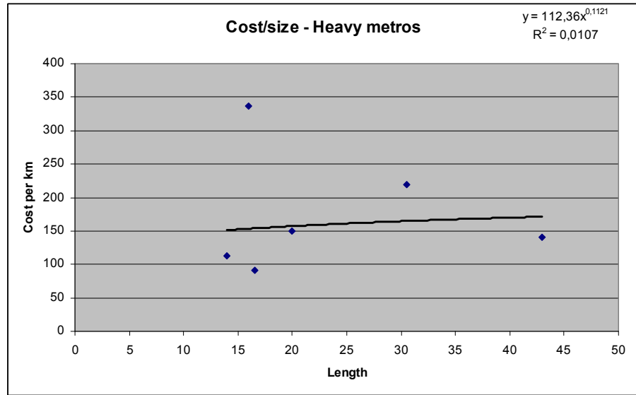
Figure A-6. Cost/size relationships for heavy tunnelled metros (based on data from Railway Technical Web Pages).
