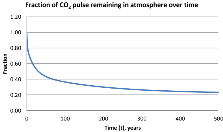
Figure 3.9: Fraction of a CO 2 pulse present in the atmosphere as a function of time. The fraction is calculated using the Bern carbon cycle, see Equation 3.7.
