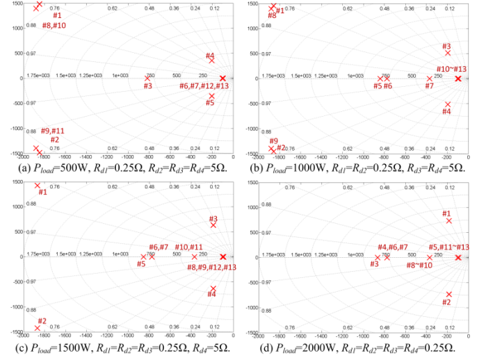
Fig. 7. Dynamic model of paralleling converter system
