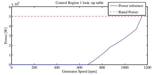
Figure 6: Power/generator-speed relationship in control region 1.
