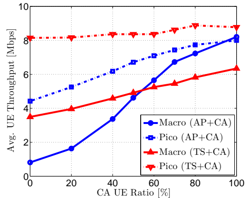
Fig. 4: Avg. UE throughput per BTS for different CA UE ratios and PCell management policies. Scenario B is assumed.
