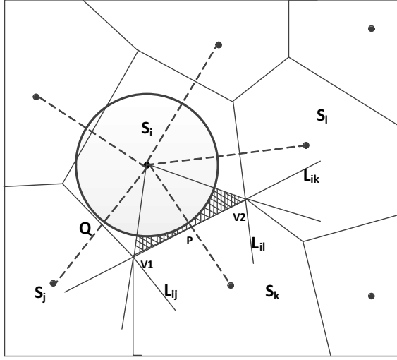
Fig. 1 Voronoi diagram for determination of coverage hole [3]
