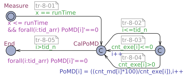
Fig. 5. PSA model of PoMD analyzer
