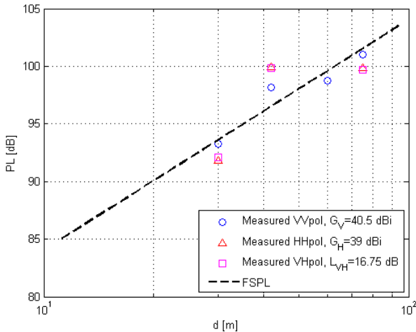
Fig. 7. Path loss in LOS conditions for the different polarization configurations, and comparison with FSPL.
