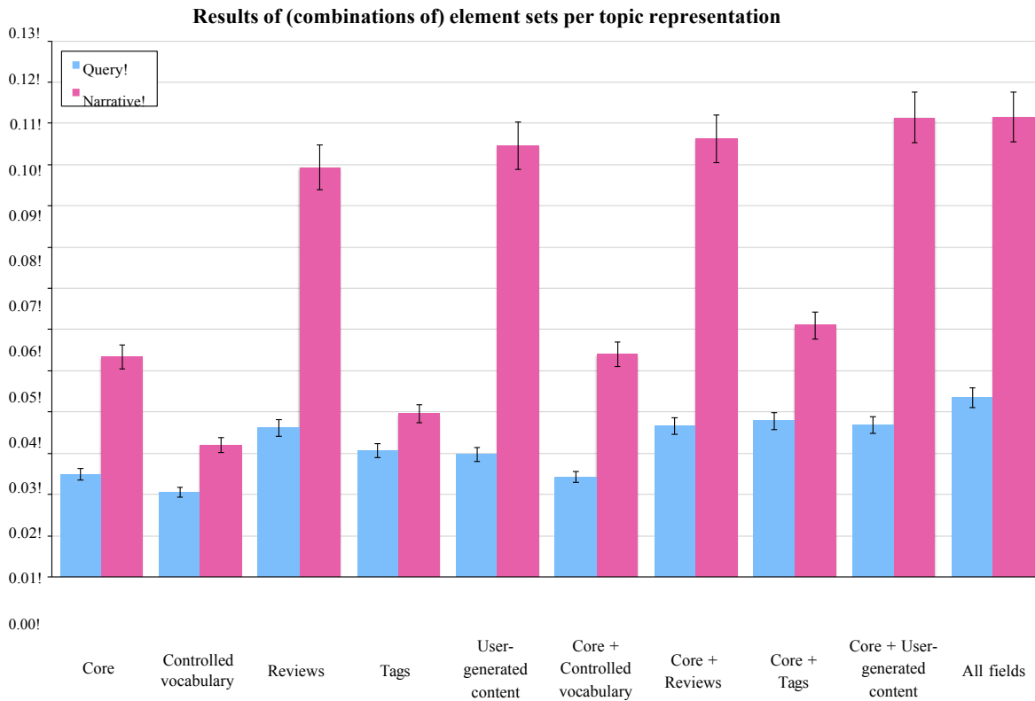
Figure 2: Results for the different metadata elements and their combination on the Any-CV collection set using NDCG@10 as evaluation metric. Bars indicate average NDCG@10 scores over 10 topics, with error bars in black.
