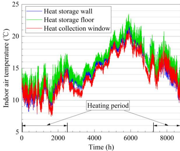
Fig. 9 Indoor air temperature for diverse designs of heat collection and storage
