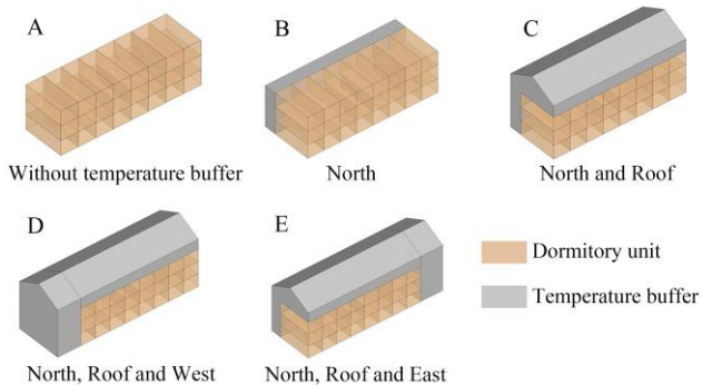
Fig. 4 Locations of temperature buffer for the dormitory
