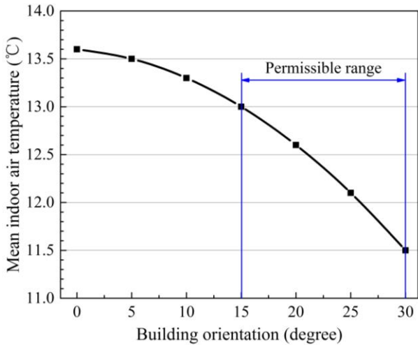
Fig. 3 Mean indoor air temperature for various building orientations
