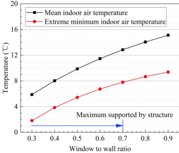
Fig. 6 Mean and extreme minimum indoor air temperatures for various window to wall ratios
