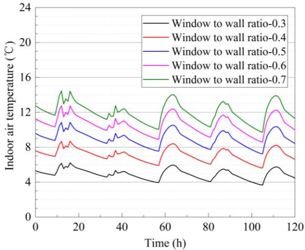
Fig. 7 Effect of window to wall ratio on indoor air temperature
