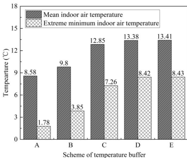
Fig. 5 Indoor air temperature for diverse schemes of temperature buffer
