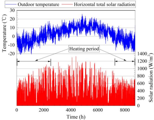
Fig. 2 Variations of weather conditions
