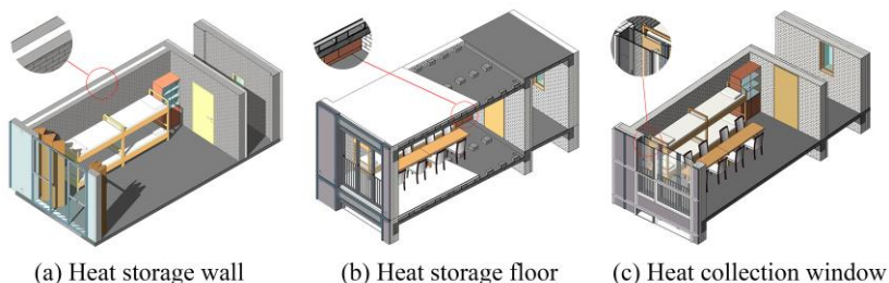
Fig. 8 Designs for heat collection and storage
