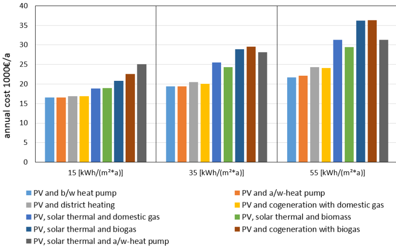
Fig. 3 Cost comparison of building systems for multi-family houses in Switzerland [8]
