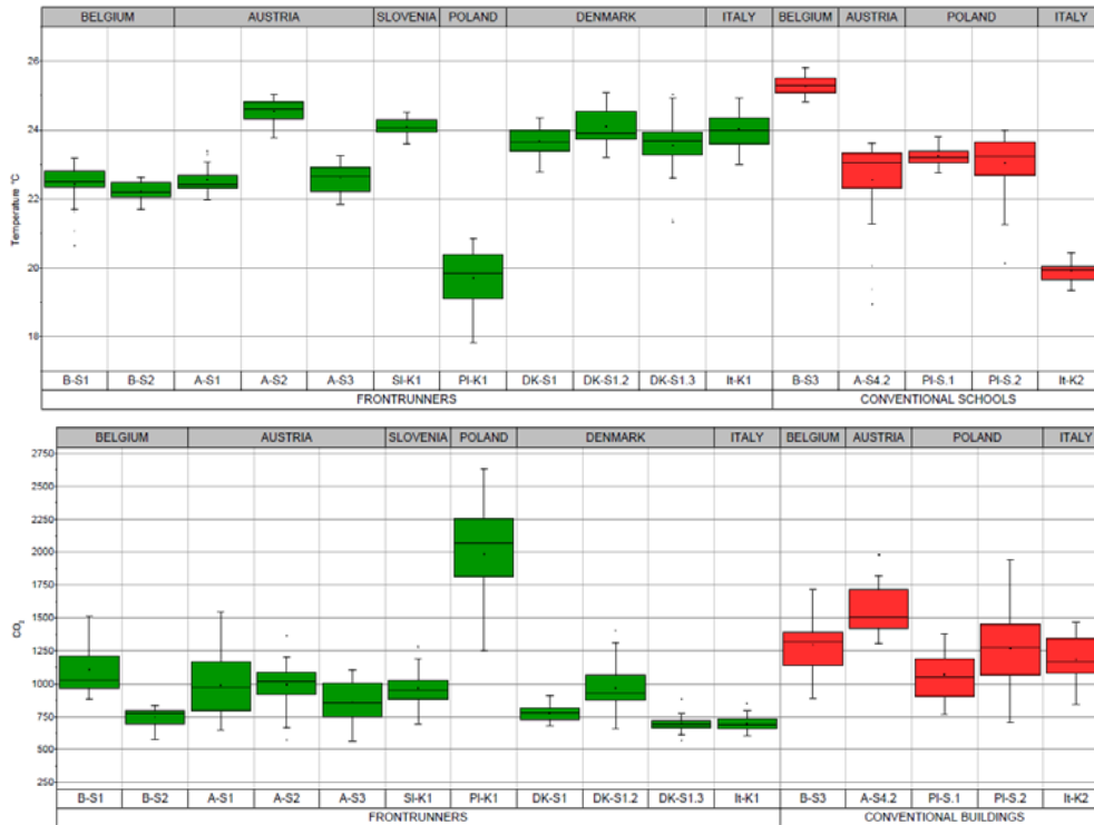
Fig. 2 Results of temperature and CO 2 measurements
