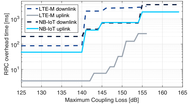
(b) Signaling overhead per packet transfer for LTE-M and NB-IoT.
