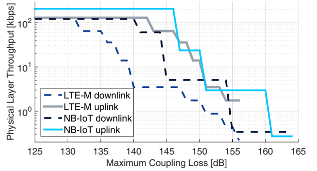
(a) Uplink and downlink physical layer throughput mapping to MCL using 1 Physical Resource Block (PRB) for LTE-M and NB-IoT.
