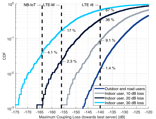
Fig. 3: MCL CDF for users in the rural area.
