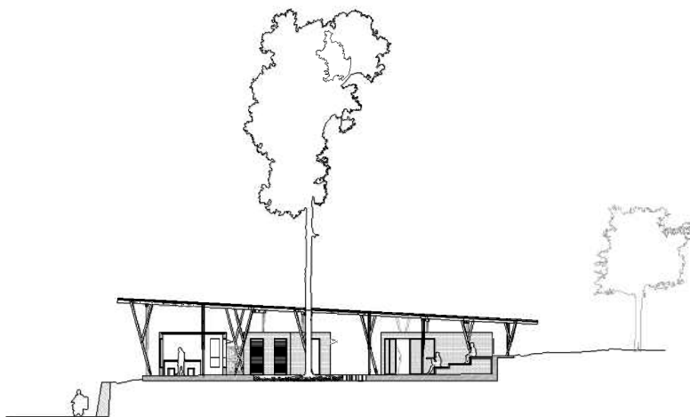
Snitt gjennom Cassia Coop Training Centre
