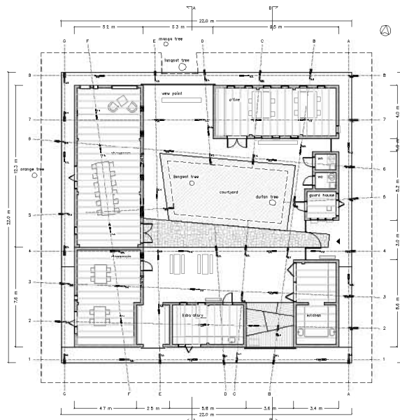
Plan Cassia Coop Training Centre
